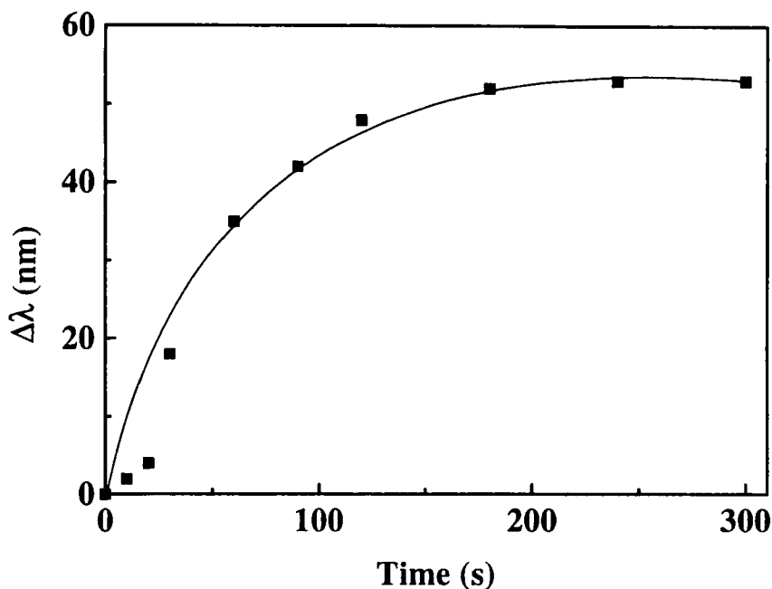
FIGURE 3 Change of reflectance band ( \Delta\lambda ) of eutectic mixture of 3a on irradiation time at 60 °C
