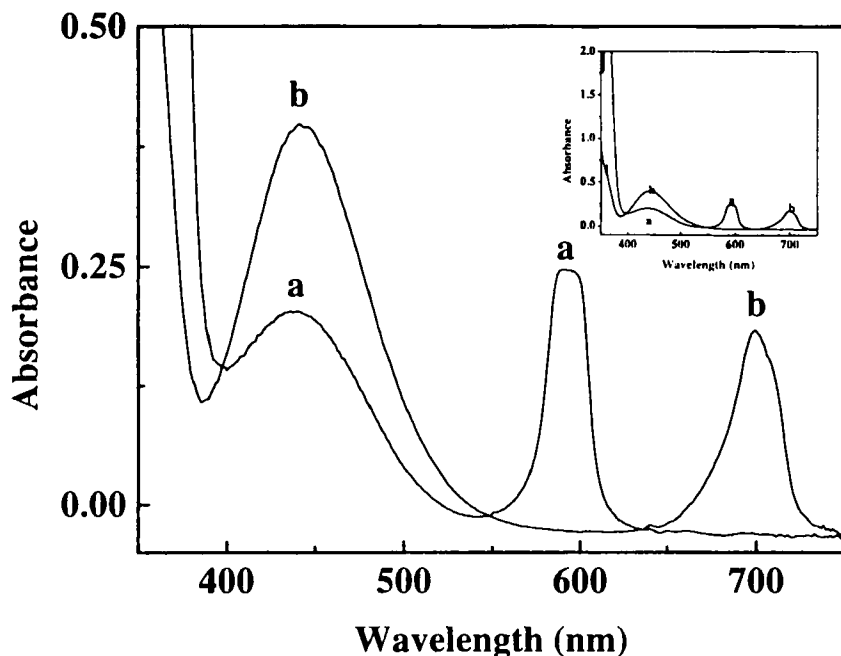
FIGURE 2 Absorption spectra of eutectic mixture of 5b; (a) before irradiation and (b) after irradiation
