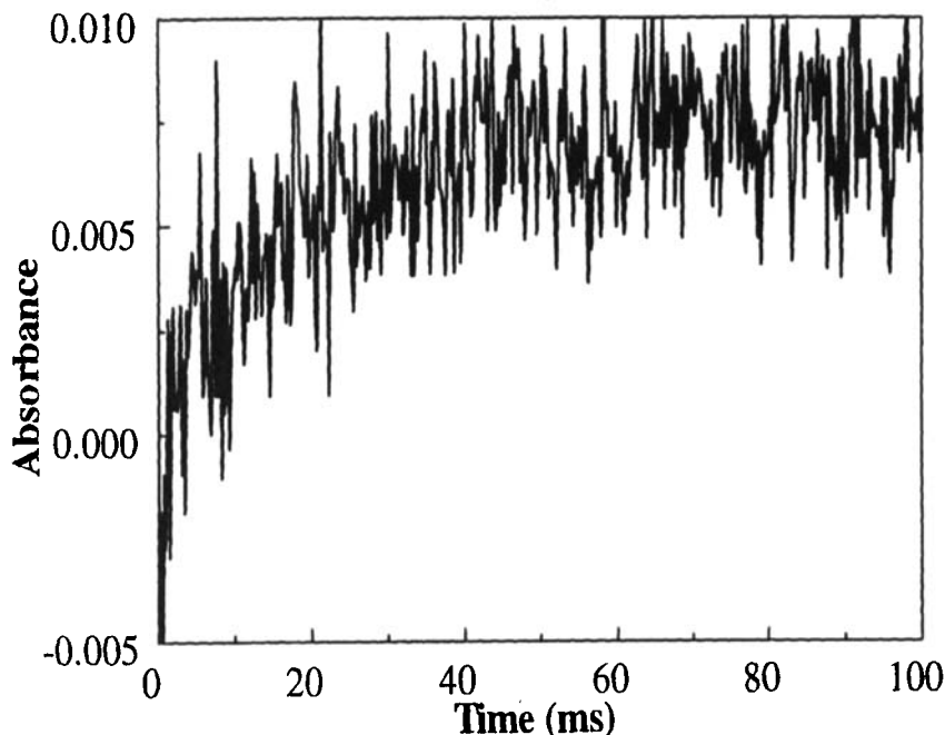
FIGURE 4 Growth of reflectance band at 600 nm measured by pulsed irradiation of eutectic mixture of 5b at 355 nm
